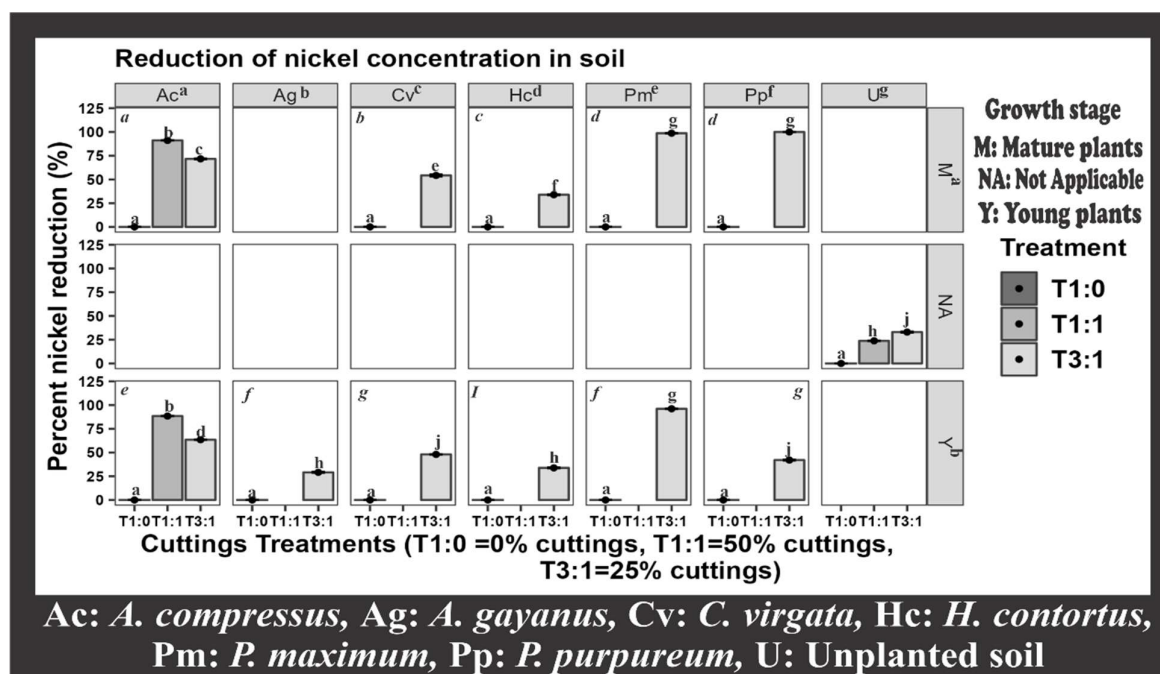
Figure 3: Percent nickel concentration reduction in soils
